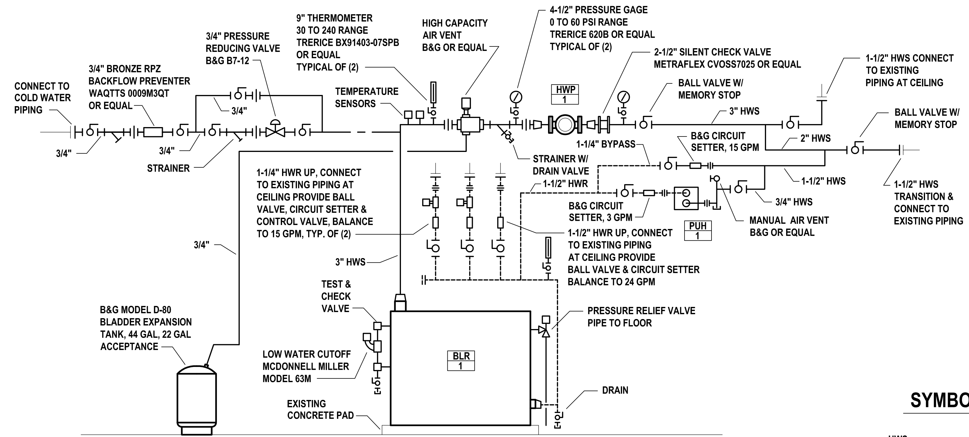
SCHEMATIC HOT WATER PIPING DIAGRAMS NO SCALE
