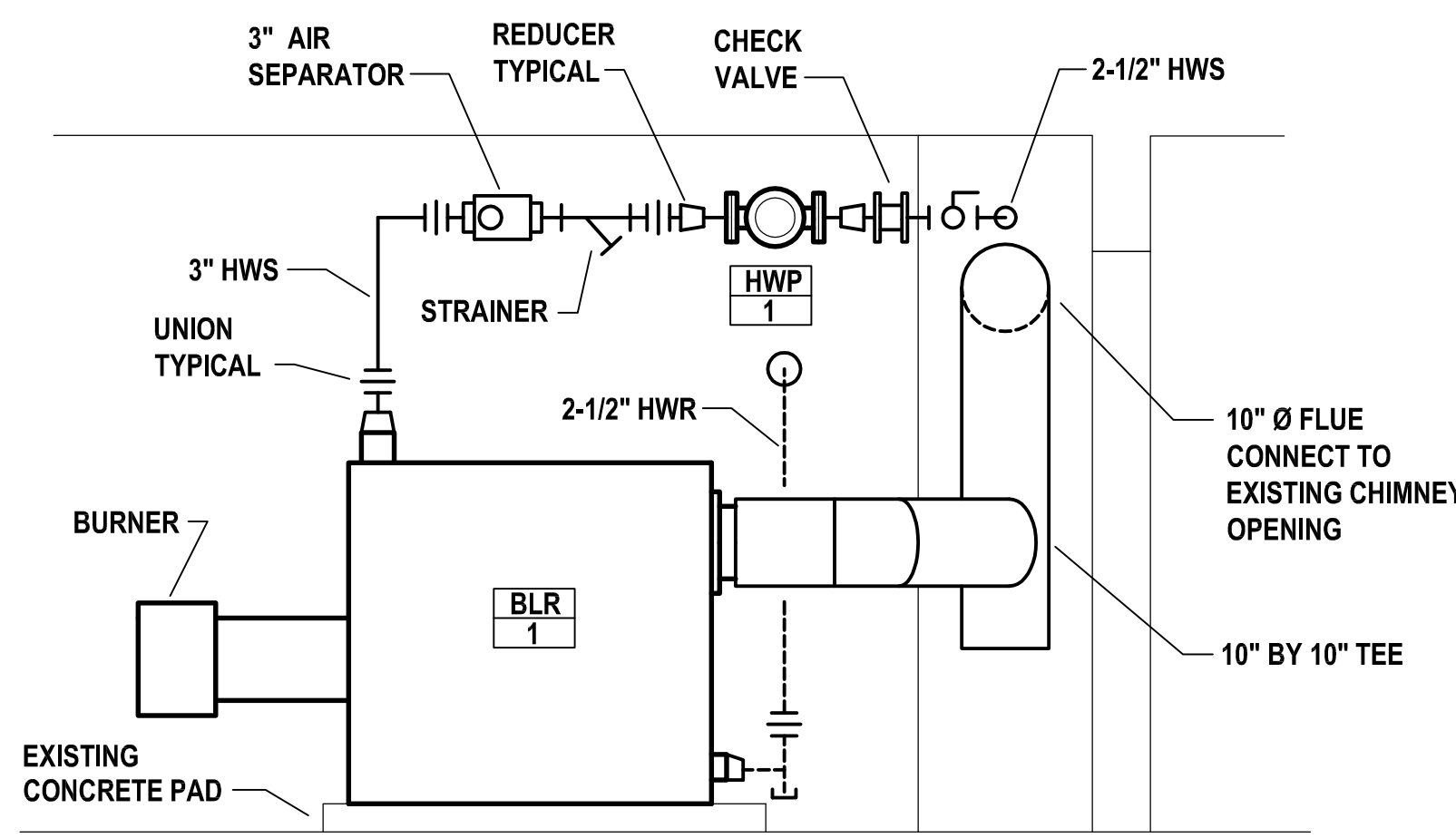
SECTION "A" BOILER ELEVATION SCALE : 1/2" = 1' - 0"
