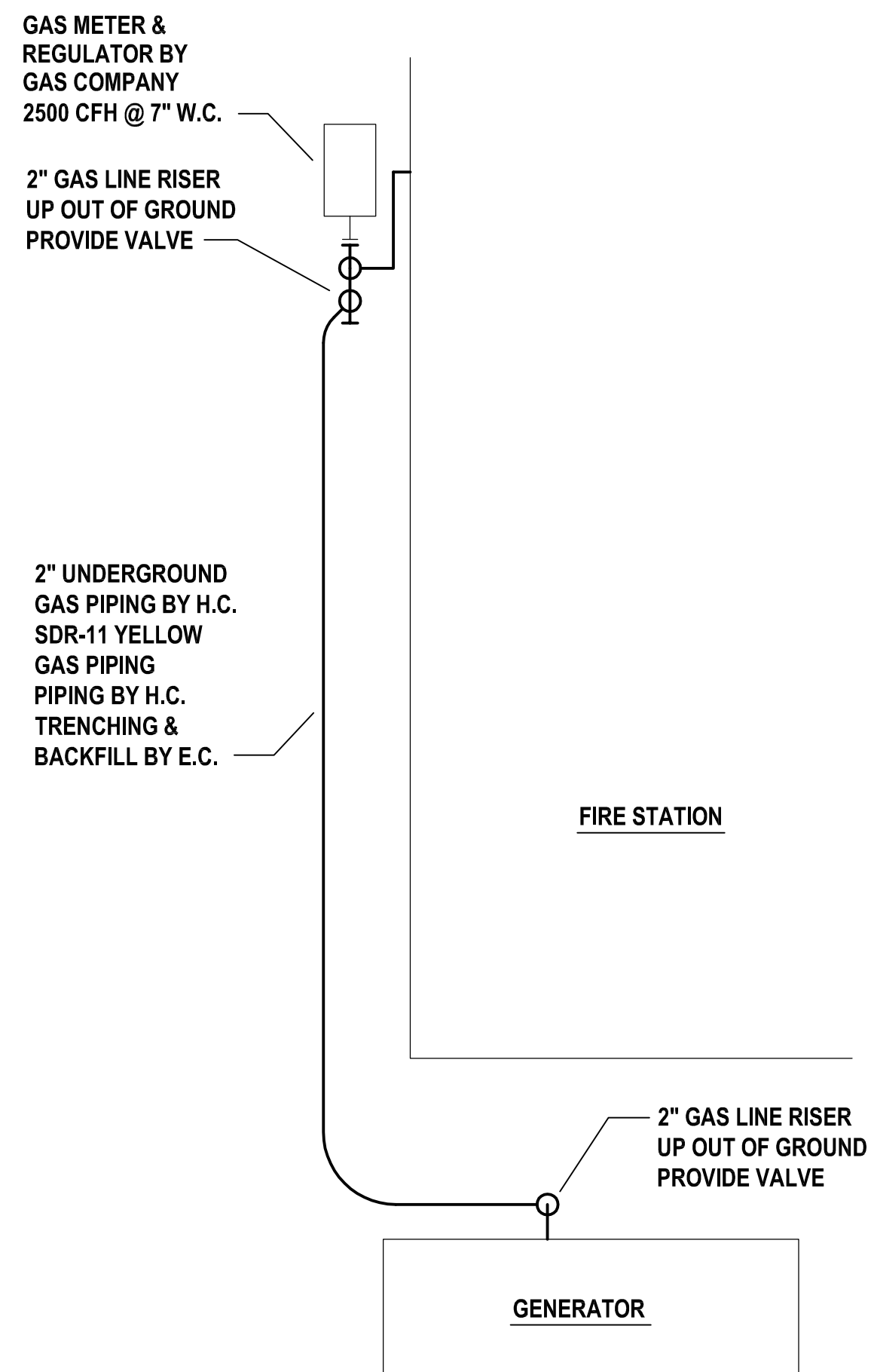
PARTIAL SITE PLAN SCALE : 1/4" = 1' - 0"
