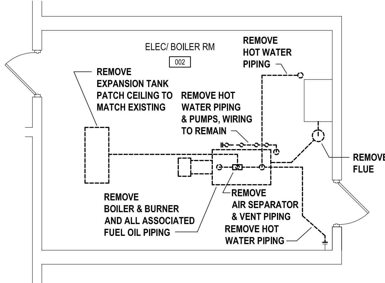
BOILER ROOM DEMOLITION PLAN SCALE : 1/4" = 1' - 0"
